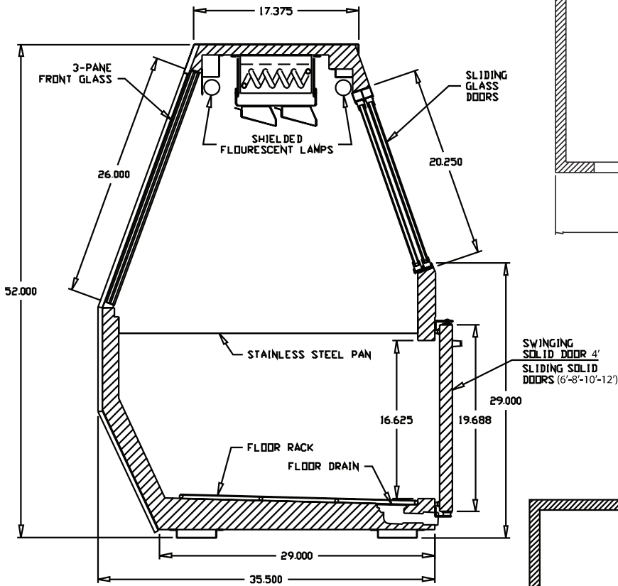
Cross Section
