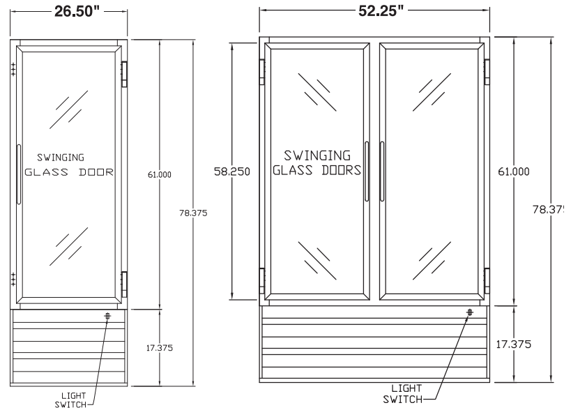
Front Views
