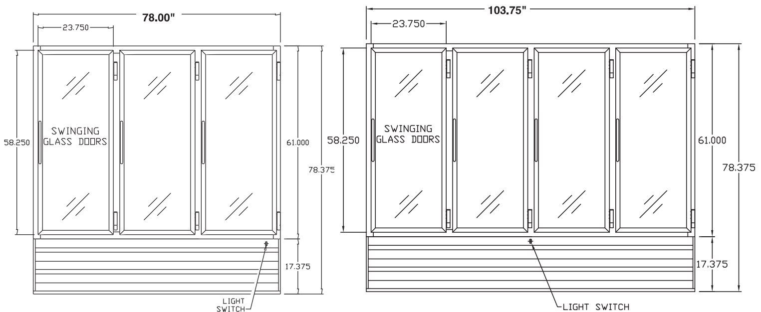
Front Views
