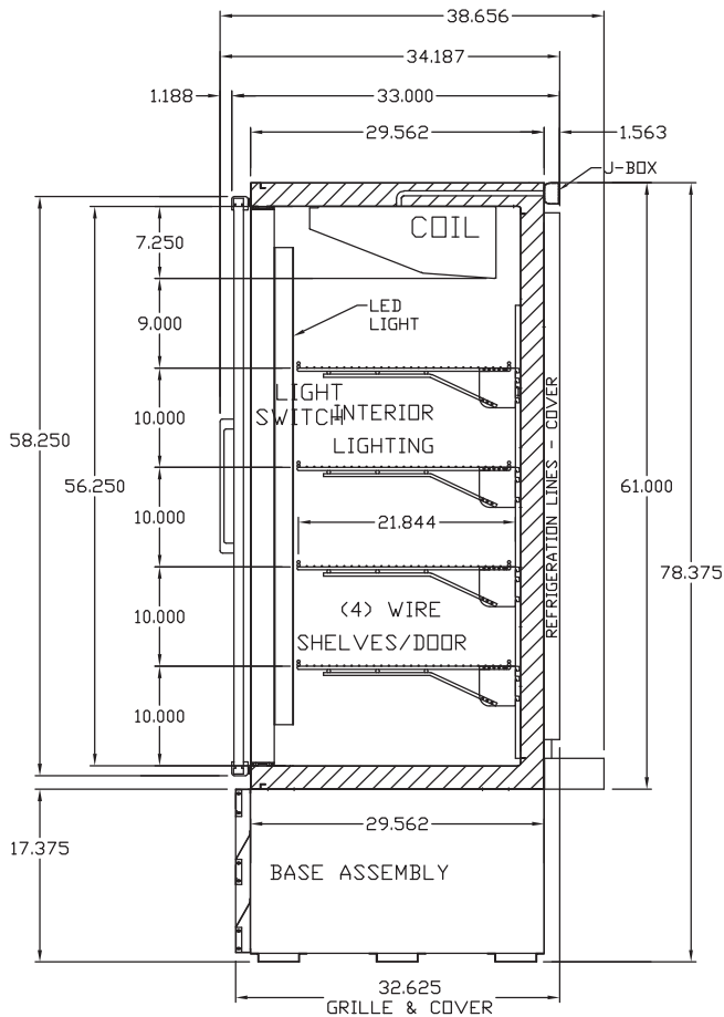
Cross Section
