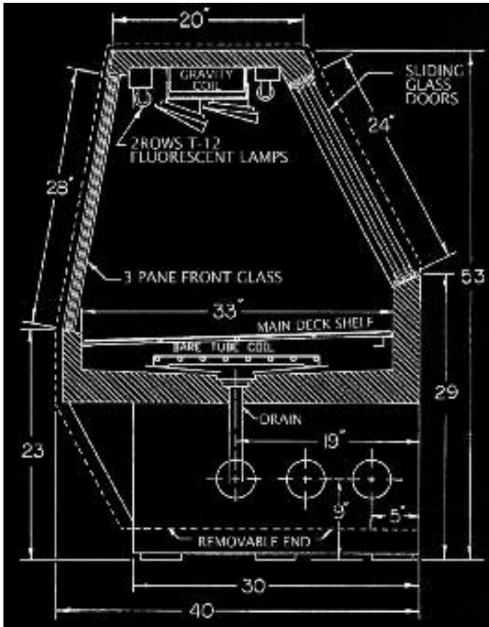
Cross Section
